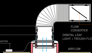
LIGHT + THROUGH FLOW - WITH TRIM (ventilation + honeycomb)
