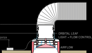
LIGHT + FLOW CONTROL - WITH TRIM (ventilation + adjuster)
