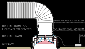
LIGHT + FLOW CONTROL - TRIMLESS (ventilation + adjuster)
