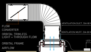
LIGHT + THROUGH FLOW - TRIMLESS (ventilation + honeycomb)
